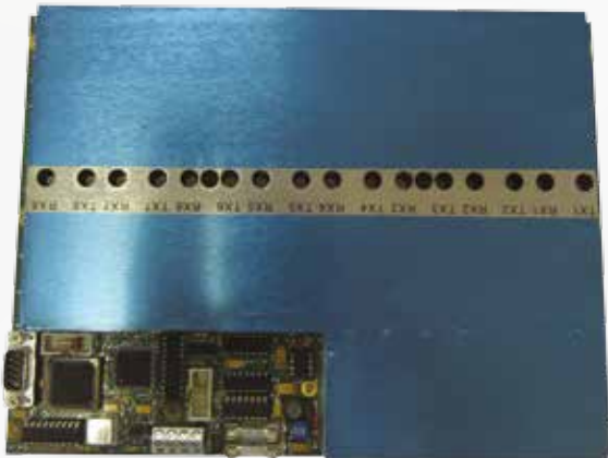
8 Independent remote pulsers attenuators & preamplifier.
